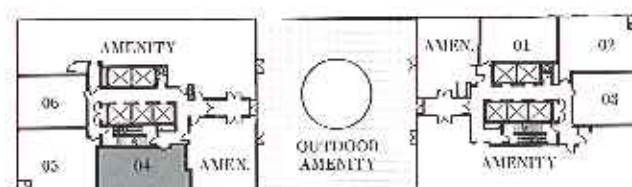
FLOOR 10
